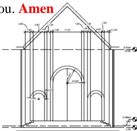
② Section 1 3/16" = 1'-0"
