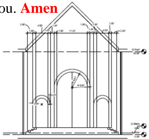
② Section 1 3/16" = 1'-0"
